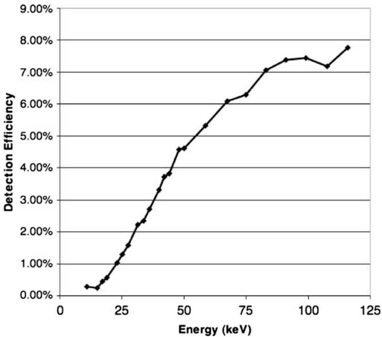
Figure 7 Efficiency, defined as the number of counts recorded by the detectors as a fraction of the number of x-ray inputs, shown as a function of input x-ray energy
