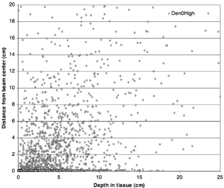
Figure 9 Distance in tissue from beam center where x-rays forming the image have an interaction, high kilovoltage
