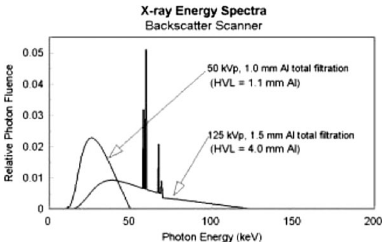
Figure 2 Published x-ray spectra for low and high kilovoltage units, from Refs. (National Council on Radiation Protection and Measurements 2003a, 2003b)
