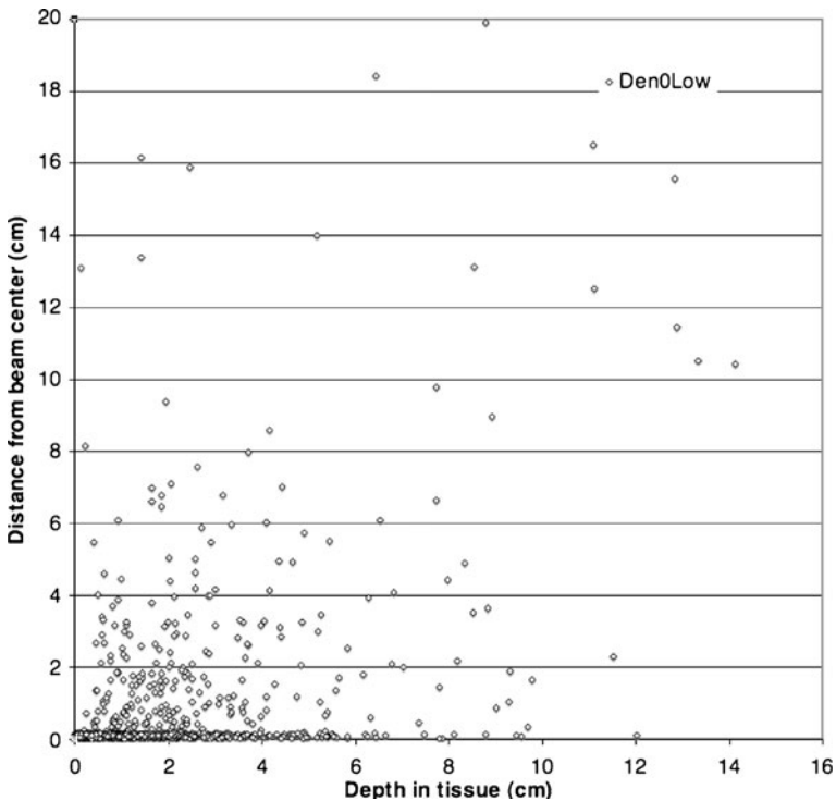
Figure 10 Distance in tissue from beam center where x-rays forming the image have an interaction, low kilovoltage
