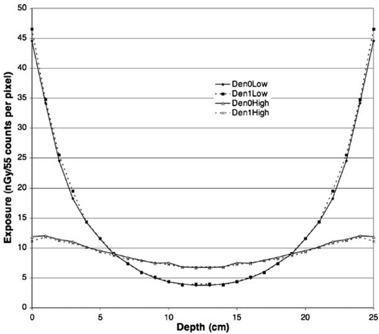
Figure 6 Same data as in Figure 5 but summed so as to simulate the exposure of a 25 cm thickness of tissue
